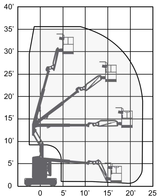
SJ30 ARJE WORKING ENVELOPE
