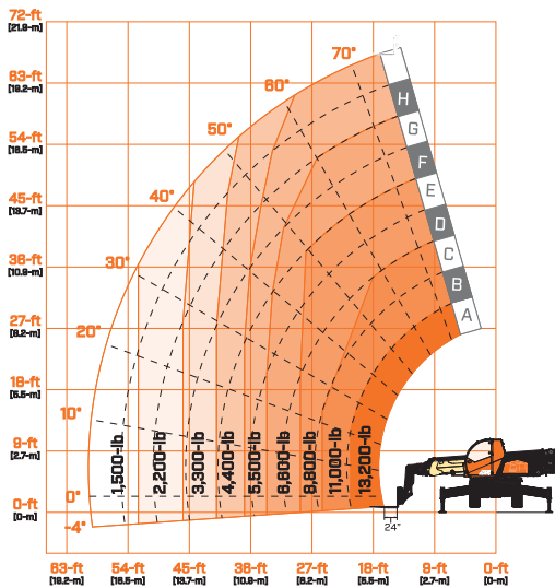
Outriggers Down
